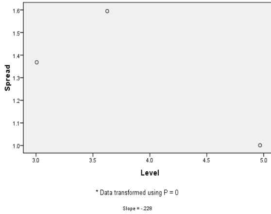
Spread vs. Level Plot of Faviidae.zn.Furmula by site
