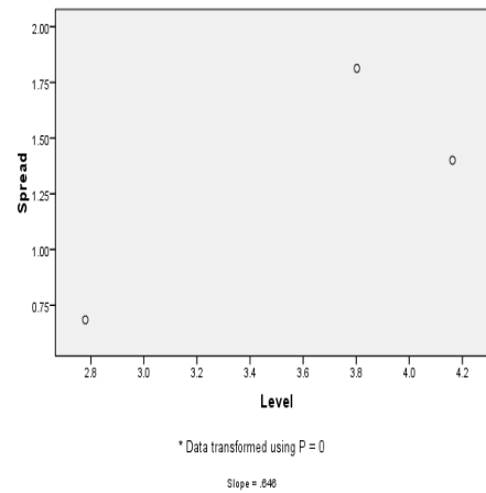
Spread vs. Level Plot of sediment.zn.Formula by site
