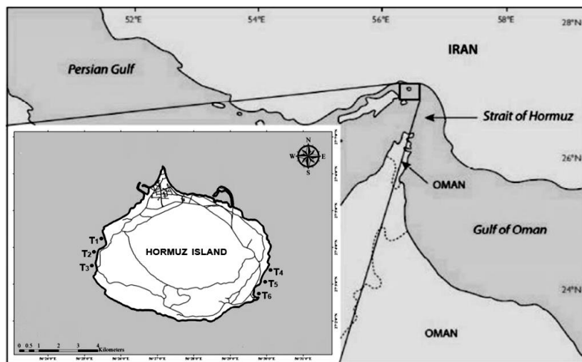
Fig. 1. Map of Hormuz Island in the Persian Gulf, showing the sampling transects
